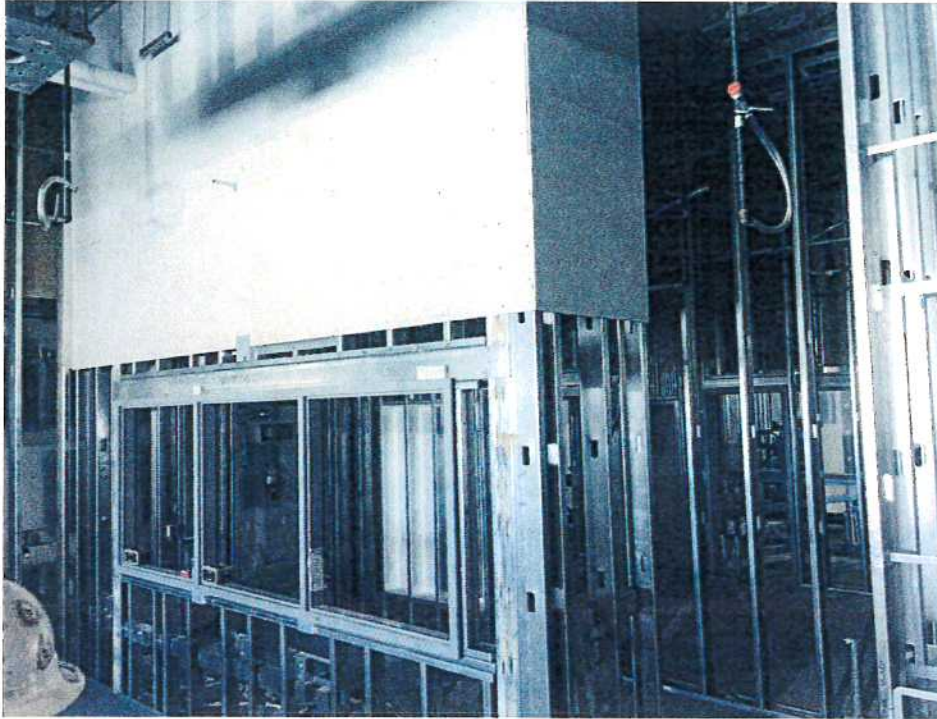
6-16-17: Top-down drywall installation in progress.
