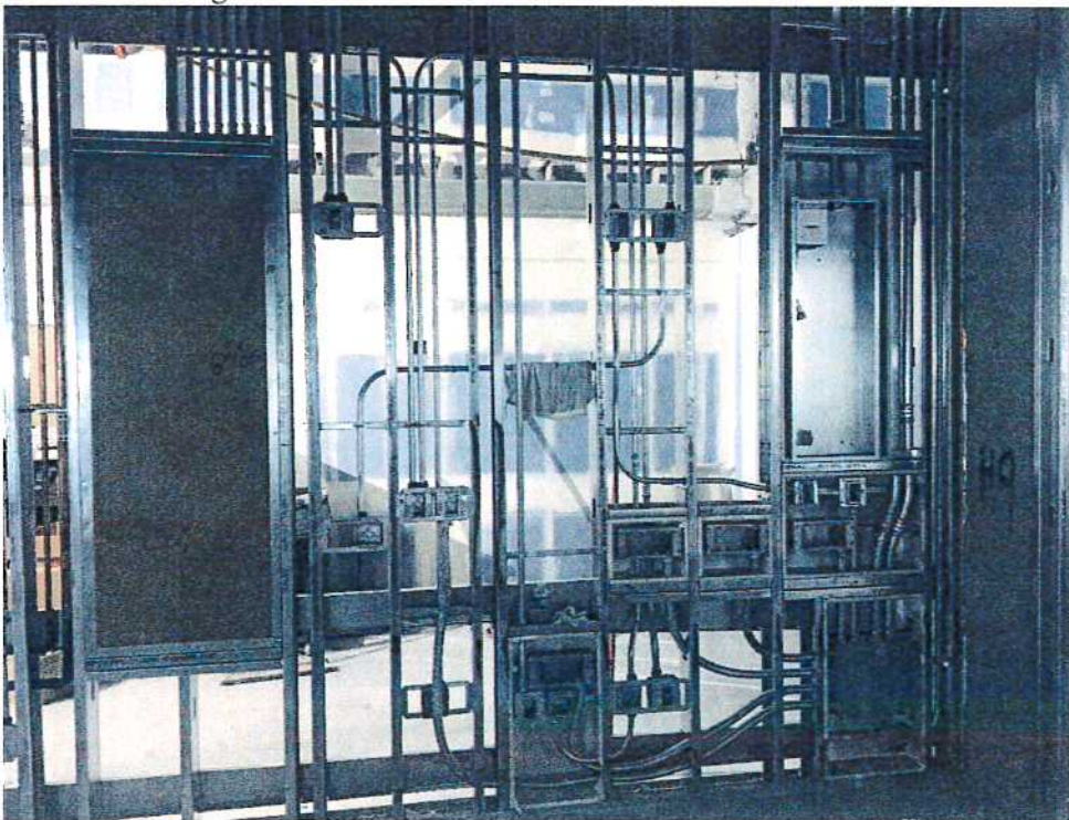
6-16-17: In wall electrical rough-in.
